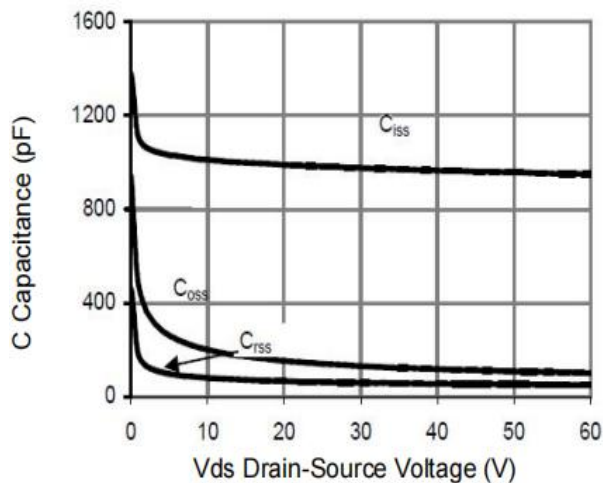
Figure 5: Capacitance Characteristics
