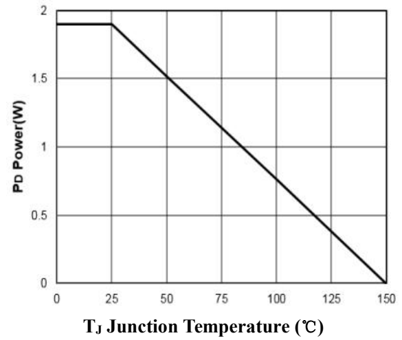
Figure 8: Power Dissipation
