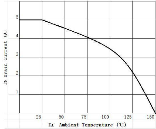
Figure 4: Drain Current vs. Temperature
