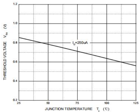
Figure 5: Threshold Voltage Characteristics
