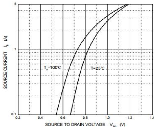
Figure 6: Diode Characteristics
