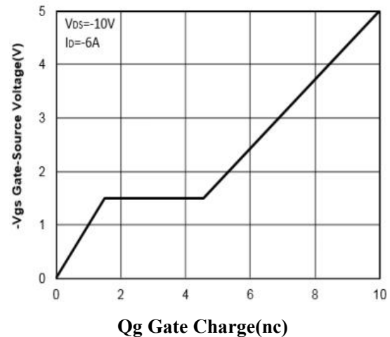
Figure 6: Gate-Charge Characteristics
