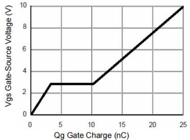
Figure 6: Gate-Charge Characteristics
