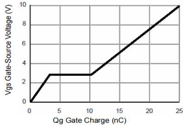
Figure 6: Gate-Charge Characteristics
