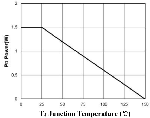
Figure 8: Power Dissipation
