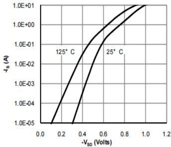
Figure 7: Diode Characteristics
