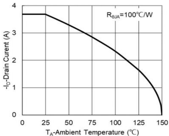
Figure 8: Drain Current vs. Temperature
