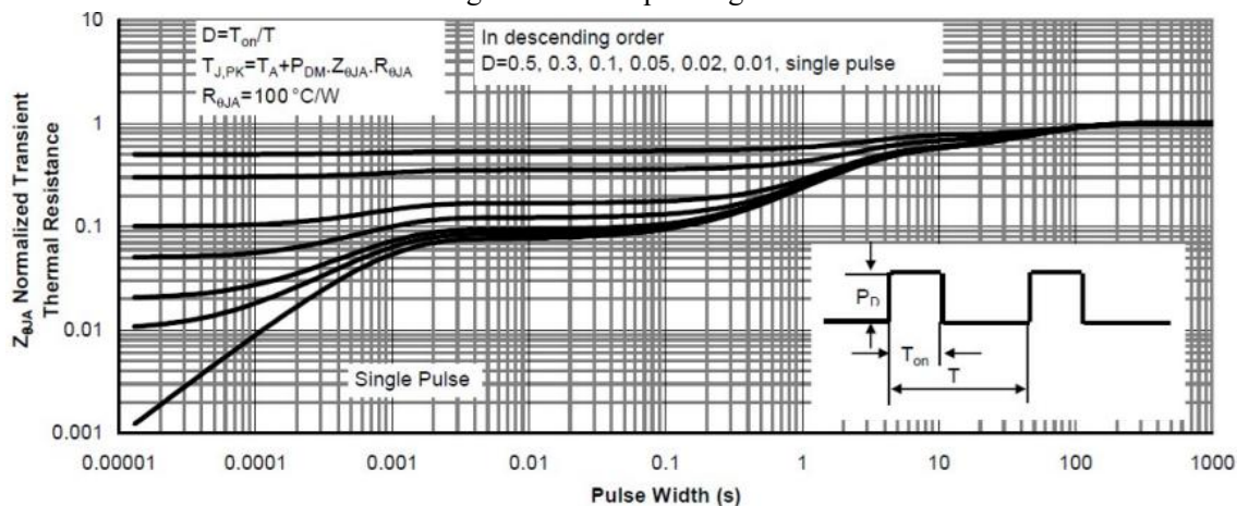
Figure 10: Transient Thermal Response Curve
