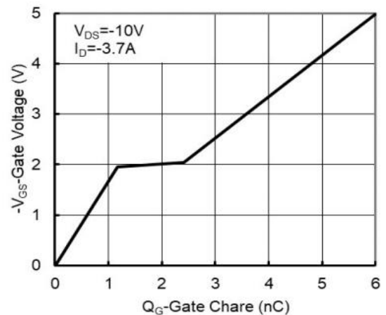
Figure 6: Gate-Charge Characteristics
