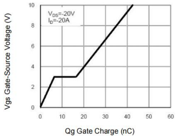
Figure 6: Gate-Charge Characteristics
