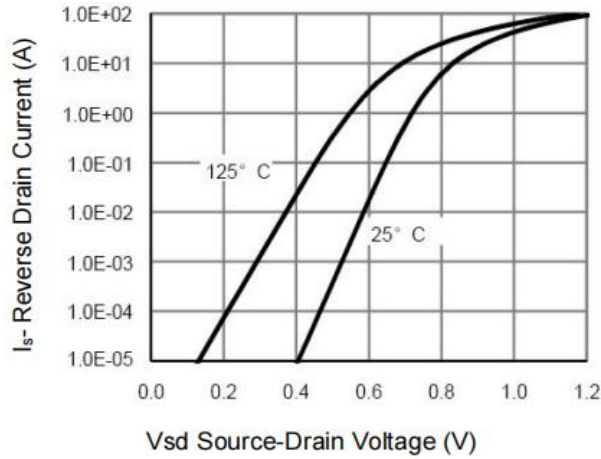
Figure 3: Diode Characteristics
