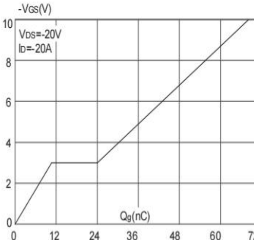
Figure 6: Gate-Charge Characteristics
