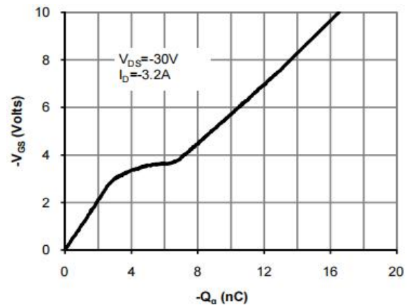
Figure 6: Gate-Charge Characteristics
