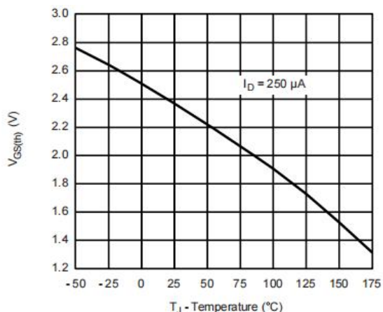
Figure 3: Threshold Voltage vs. Temperature
