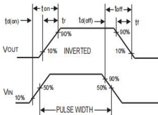
Figure 10: Switching Waveform
