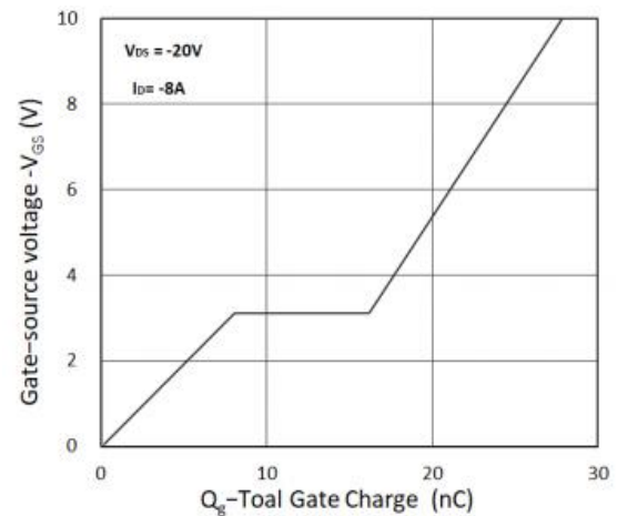
Figure 6: Gate-Charge Characteristics
