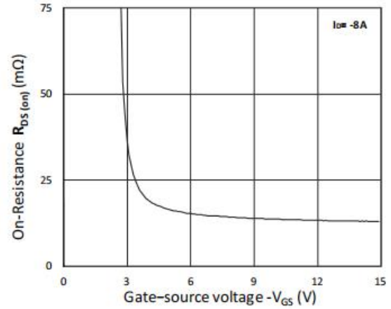
Figure 2: On-Resistance vs. V_{GS}
