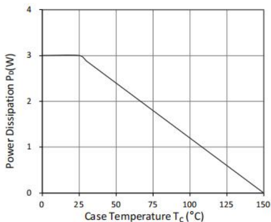
Figure 7: Power Rating Curve
