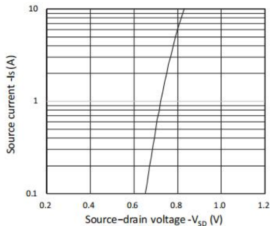
Figure 8: Diode Characteristics
