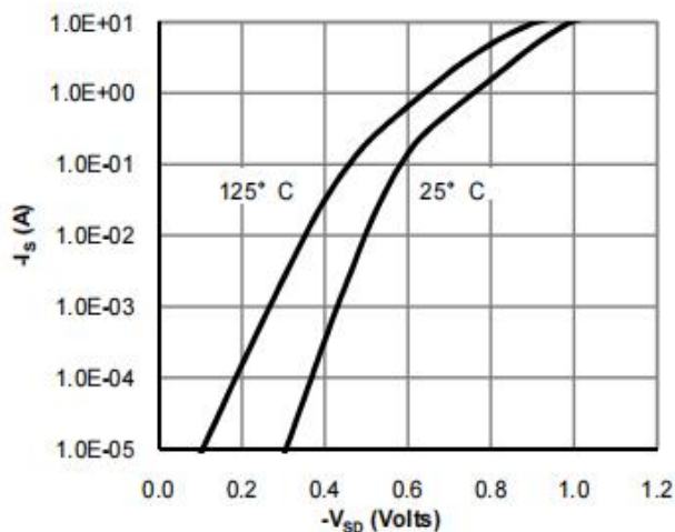
Figure 8: Diode Characteristics
