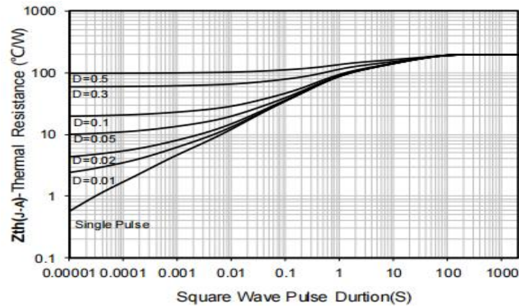
Figure 9: Transient Thermal Response Curve
