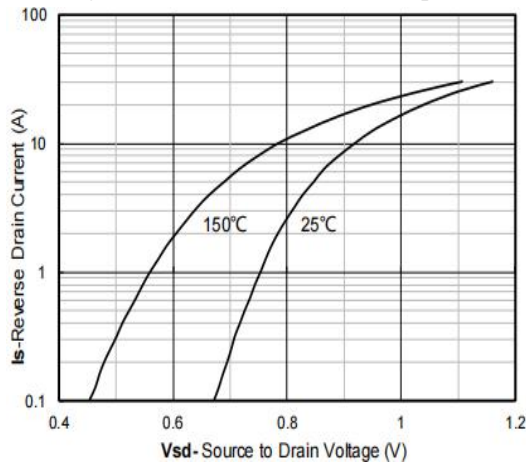
Figure 9: Diode Characteristics
