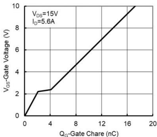
Figure 6: Gate-Charge Characteristics
