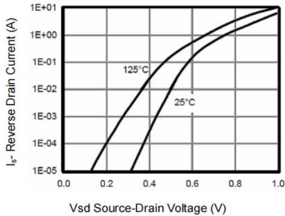
Figure 9: Diode Characteristics
