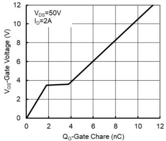
Figure 6: Gate-Charge Characteristics
