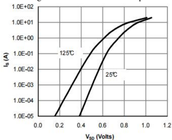
Figure 9: Diode Characteristics
