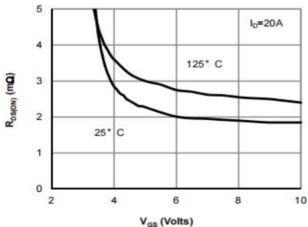
Figure 4: On-Resistance vs. V_{GS}
