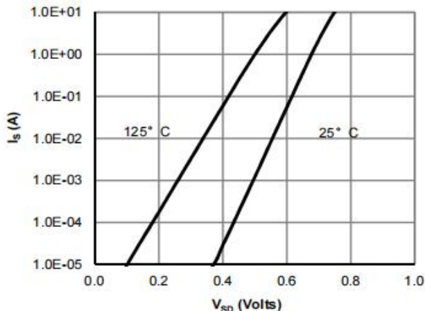
Figure 8: Diode Characteristics
