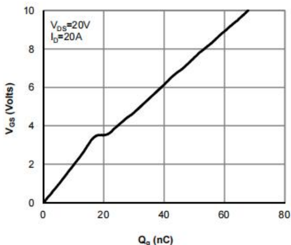
Figure 6: Gate-Charge Characteristics
