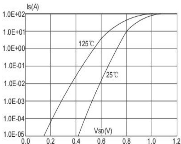
Figure 9: Diode Characteristics
