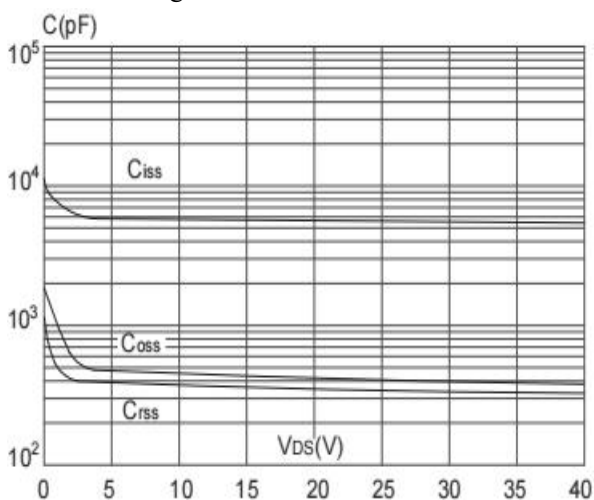
Figure 5: Capacitance Characteristics
