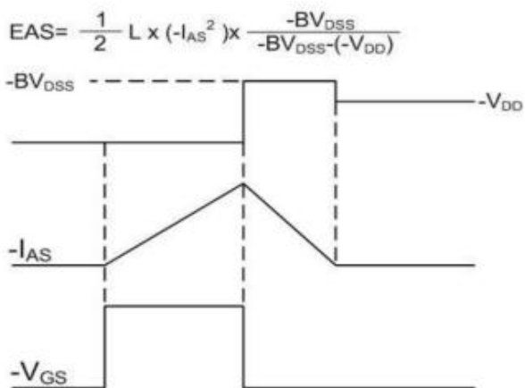
Figure 9: Unclamped Inductive Switching Waveform
