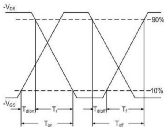
Figure 8: Switching Time Waveform
