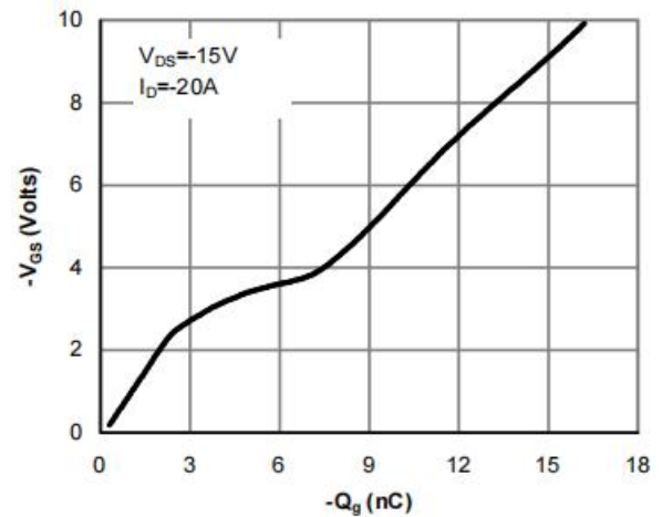
Figure 6: Gate-Charge Characteristics
