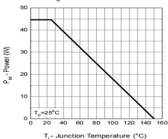
Figure 4: Power Rating Characteristics
