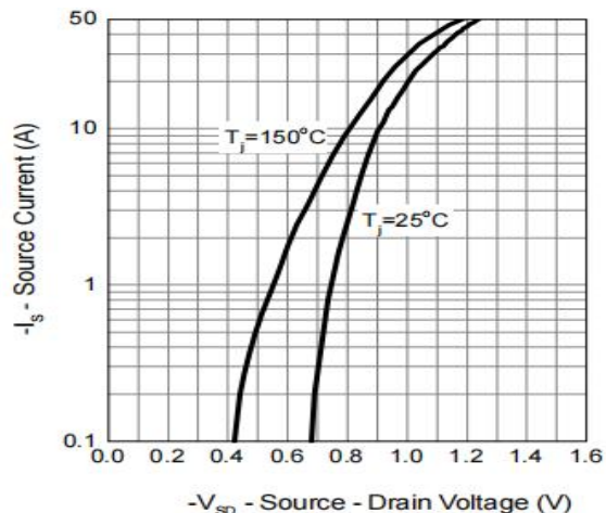
Figure 2: Diode Characteristics
