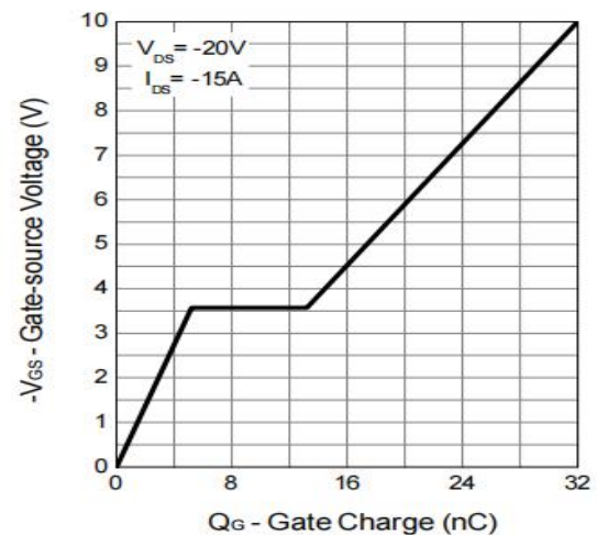
Figure 6: Gate-Charge Characteristics
