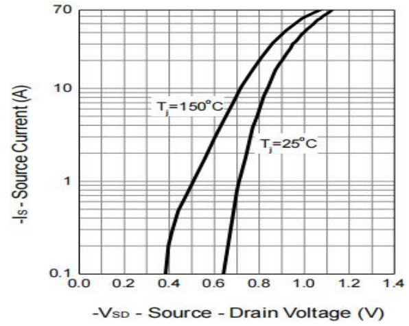
Figure 2: Diode Characteristics
