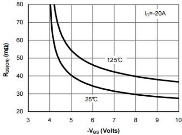
Figure 9: On-Resistance vs. Threshold Voltage
