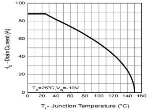
Figure 4: Drain Current vs. T_J
