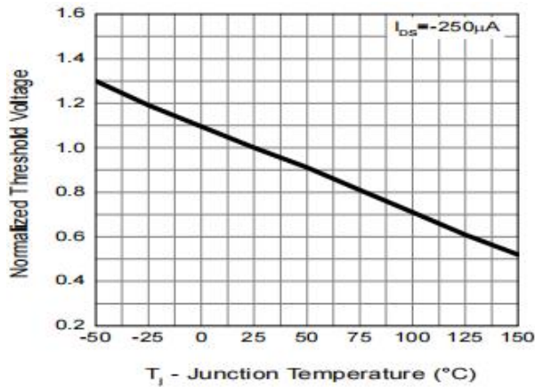
Figure 9: Threshold Voltage vs. T_J
