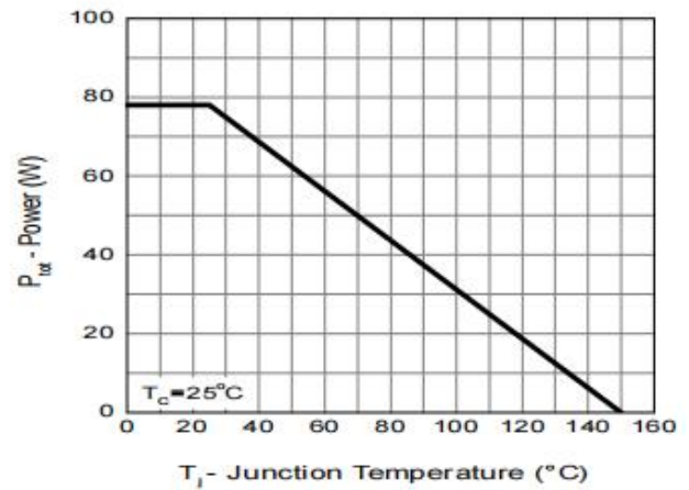
Figure 8: Power Rating Characteristics
