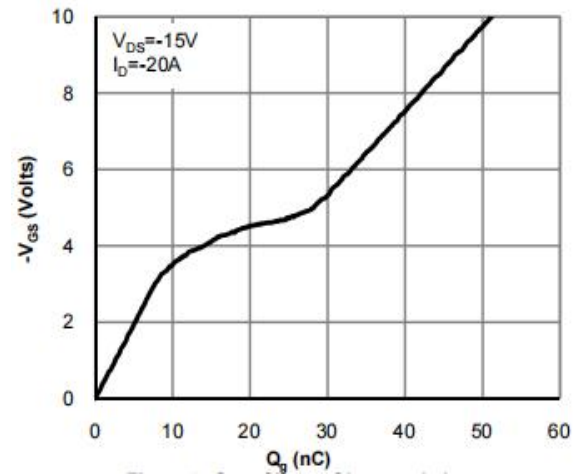
Figure 6: Gate-Charge Characteristics
