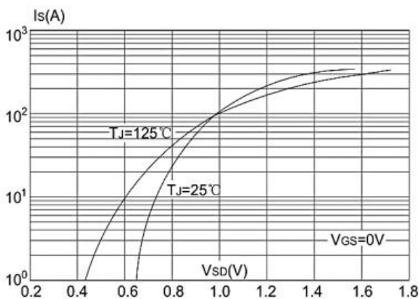
Figure 9: Diode Characteristics
