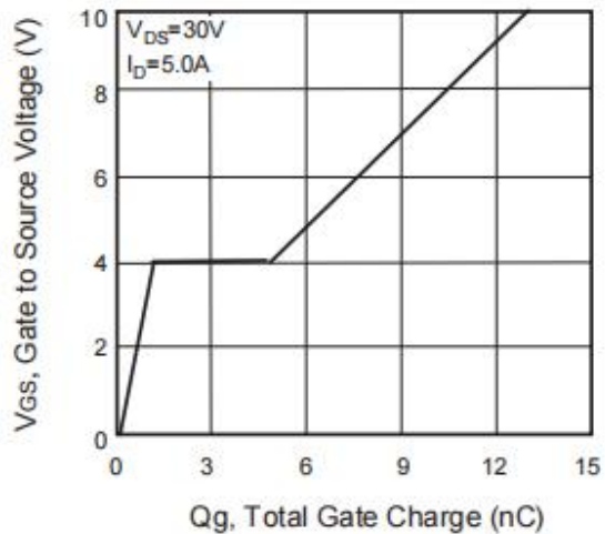
Figure 6: Gate-Charge Characteristics
