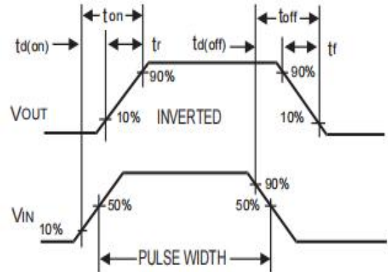
Figure 10: Switching Waveform
