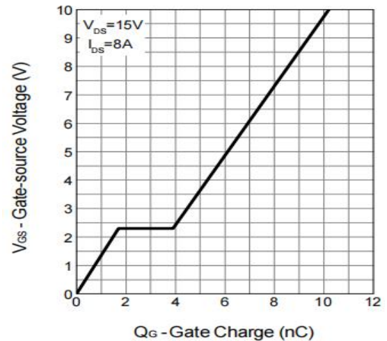
Figure 6: Gate-Charge Characteristics
