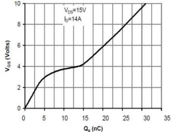
Figure 6: Gate-Charge Characteristics
