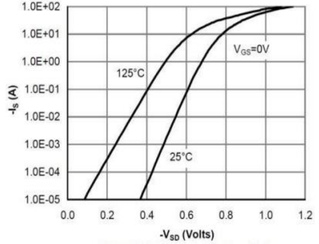
Figure 8: Diode Characteristics
