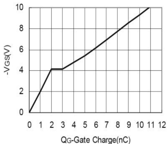
Figure 6: Gate-Charge Characteristics
