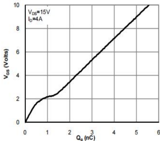
Figure 6: Gate-Charge Characteristics
