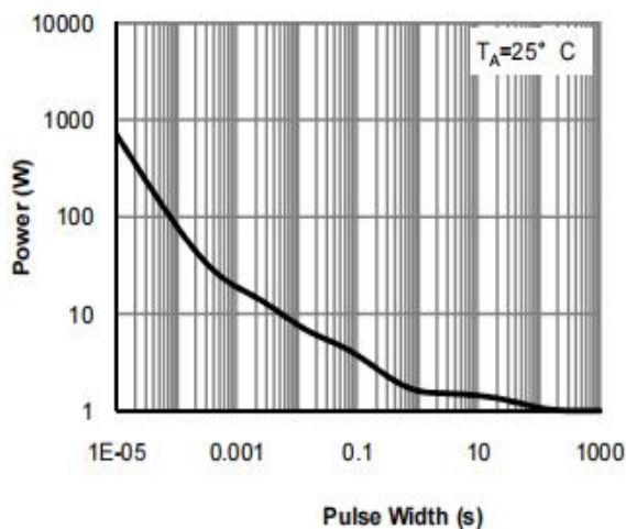
Figure 8: Power Rating
