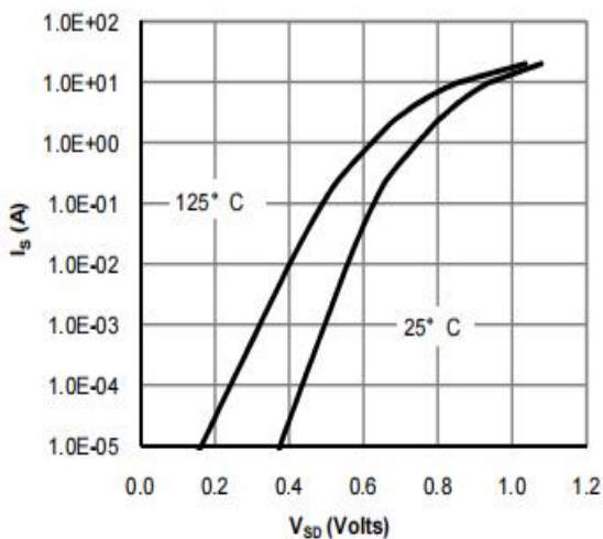
Figure 9: Diode Characteristics
