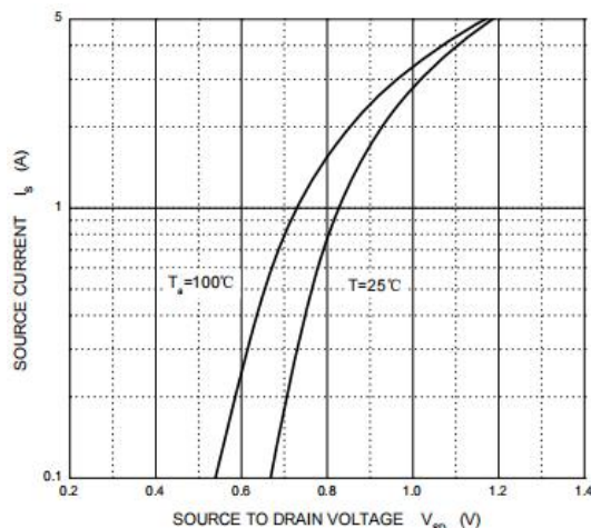
Figure 6: Diode Characteristics
