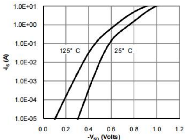
Figure 7: Diode Characteristics
