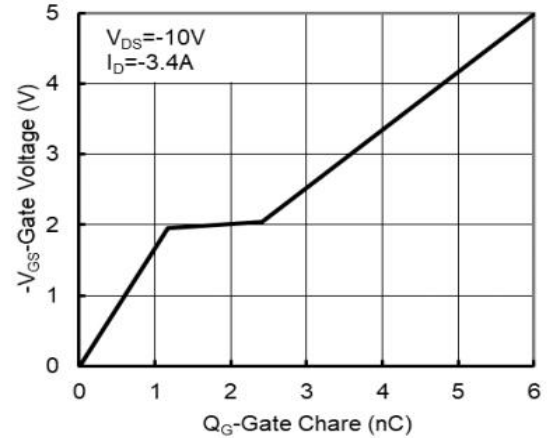
Figure 6: Gate-Charge Characteristics
