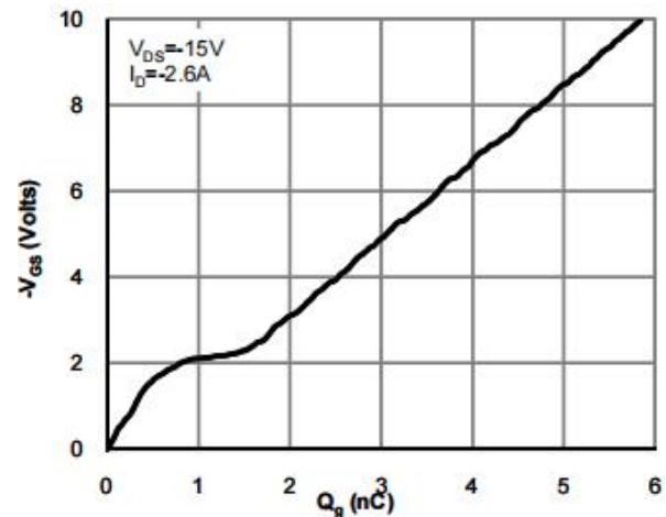
Figure 6: Gate-Charge Characteristics
