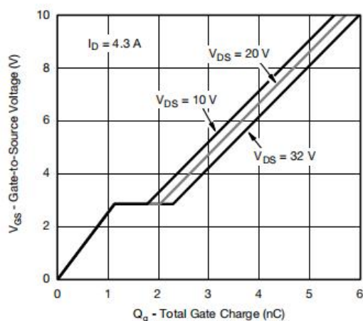
Figure 6: Gate-Charge Characteristics
