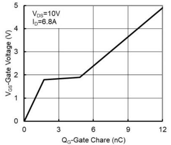
Figure 6: Gate-Charge Characteristics
