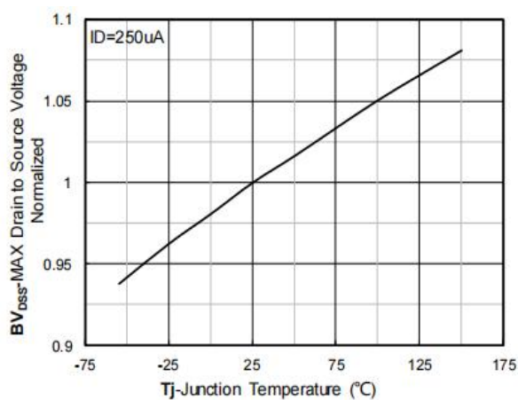
Figure 8: Breakdown Voltage vs. Temperature
