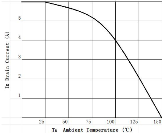
Figure 7: Drain Current vs. Temperature
