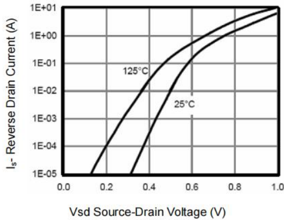
Figure 9: Diode Characteristics
