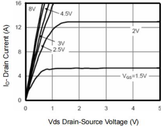
Figure 1: Output Characteristics
