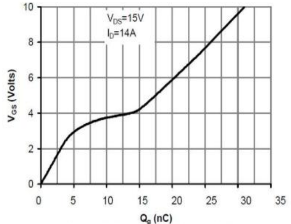
Figure 6: Gate-Charge Characteristics
