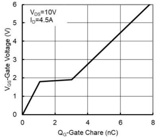
Figure 6: Gate-Charge Characteristics
