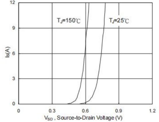
Figure 2: Forward Characteristics
