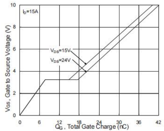
Figure 6: Gate-Charge Characteristics
