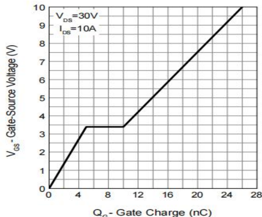
Figure 6: Gate-Charge Characteristics
