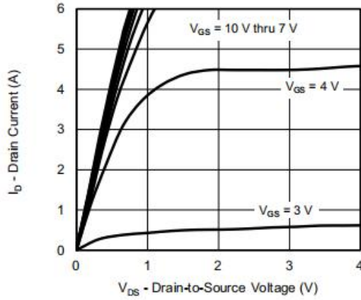
Figure 1: Output Characteristics
