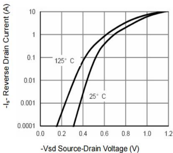
Figure 9: Diode Characteristics
